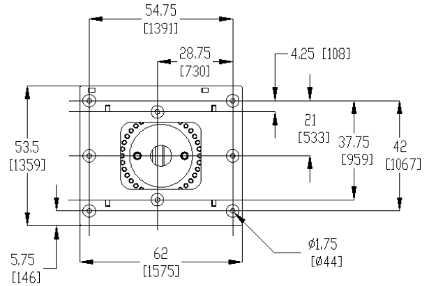
Pedestal Base Dimension: MRHT16 - MRHT20 - MRHT2025 - MRHT25
